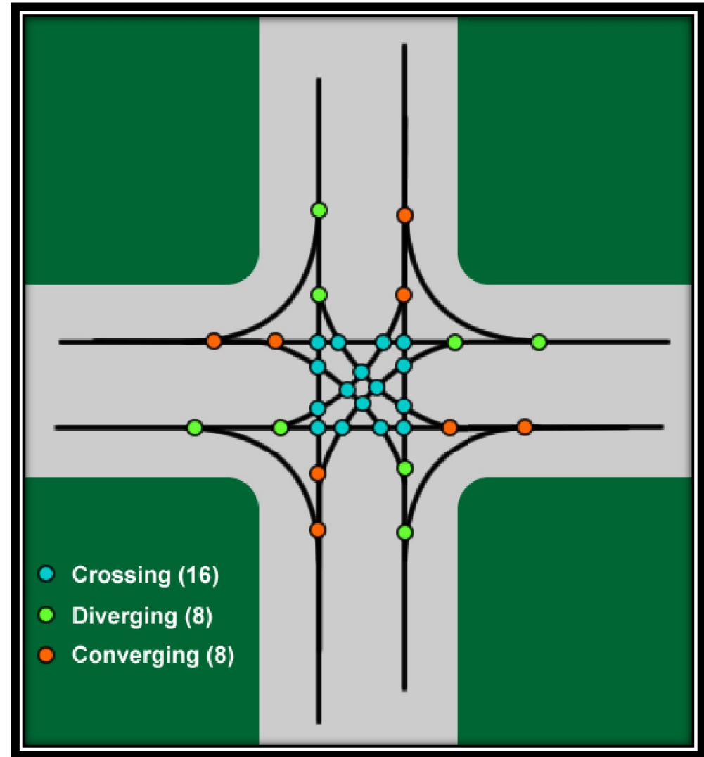
32 Conflict Points
