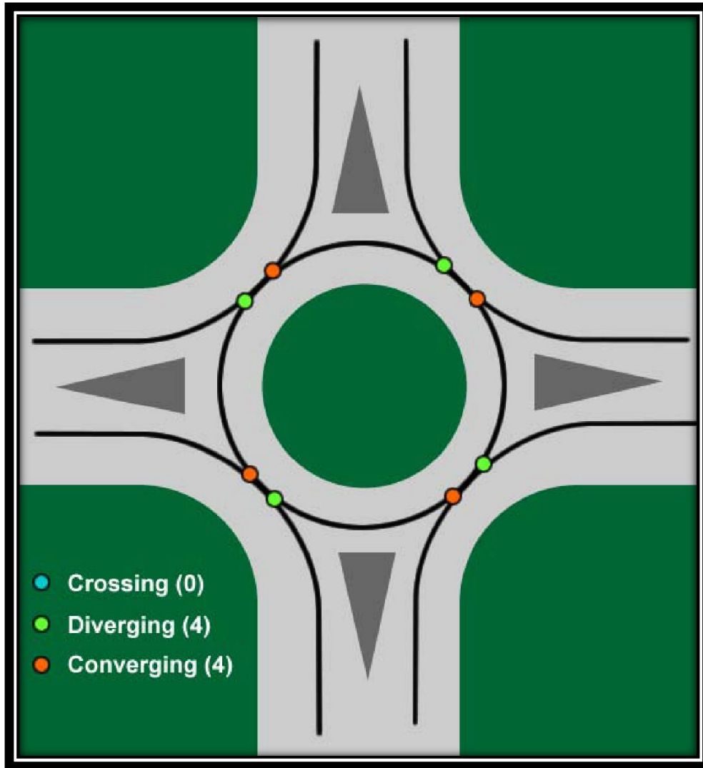
8 Conflict Points
