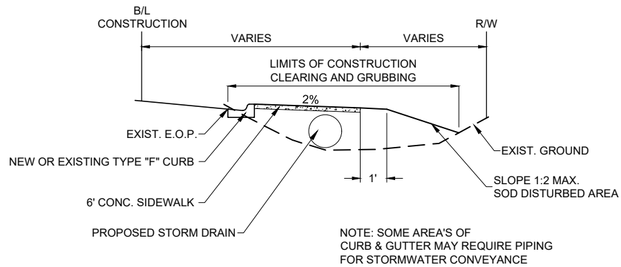
TYPICAL SECTION
