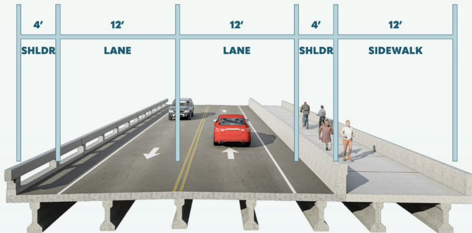
ALTERNATIVE 2 Bridge Widening
