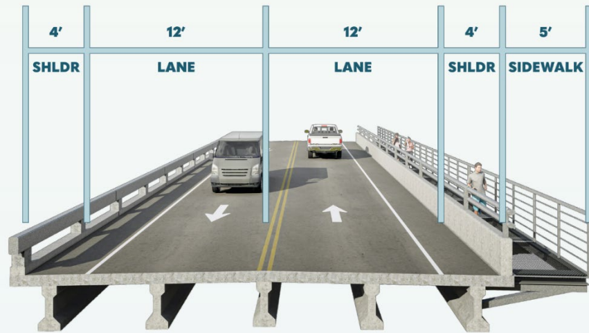
ALTERNATIVE 1 Cantilever Bridge Deck Panels
