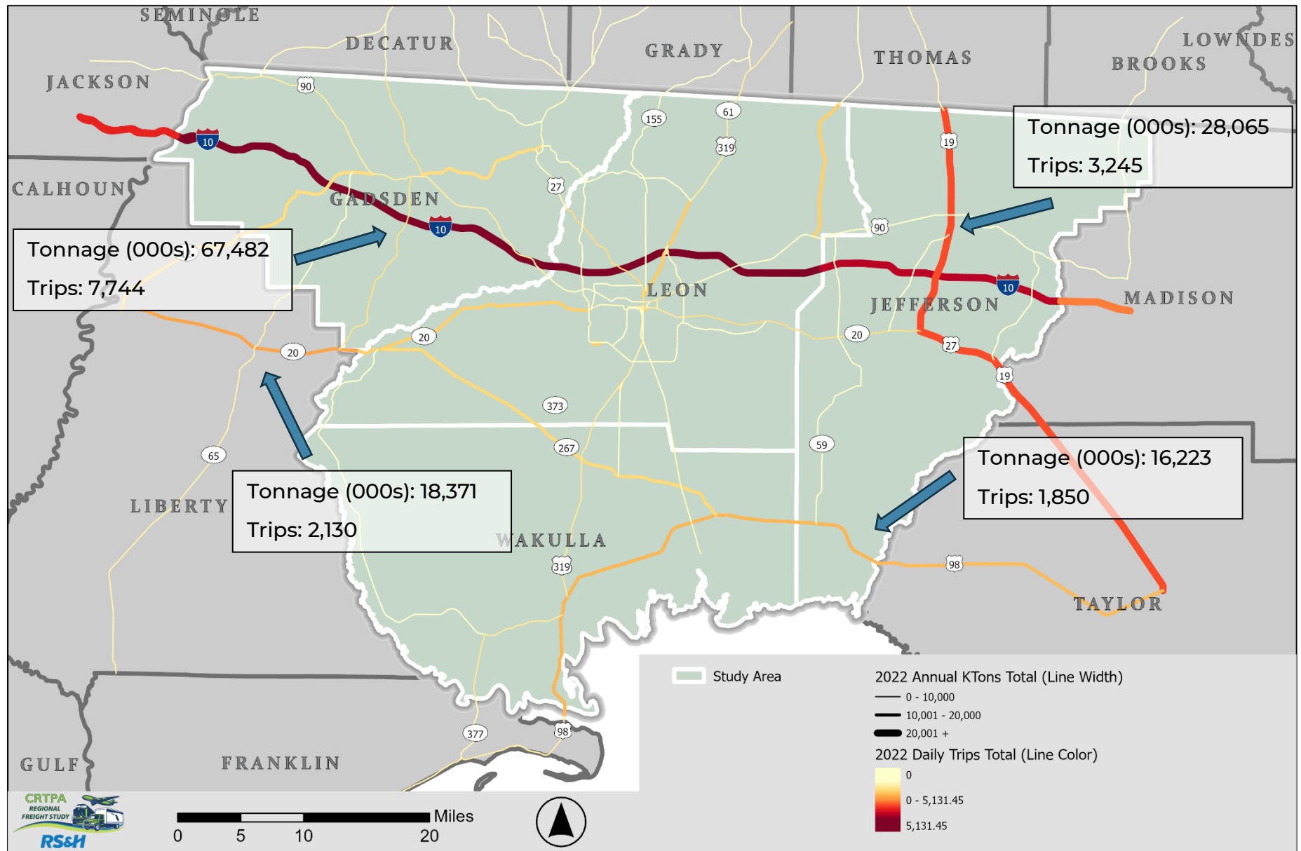
Figure 26: Annual Freight Volume (thousand tons) and Daily Trips by Corridor (2022)
