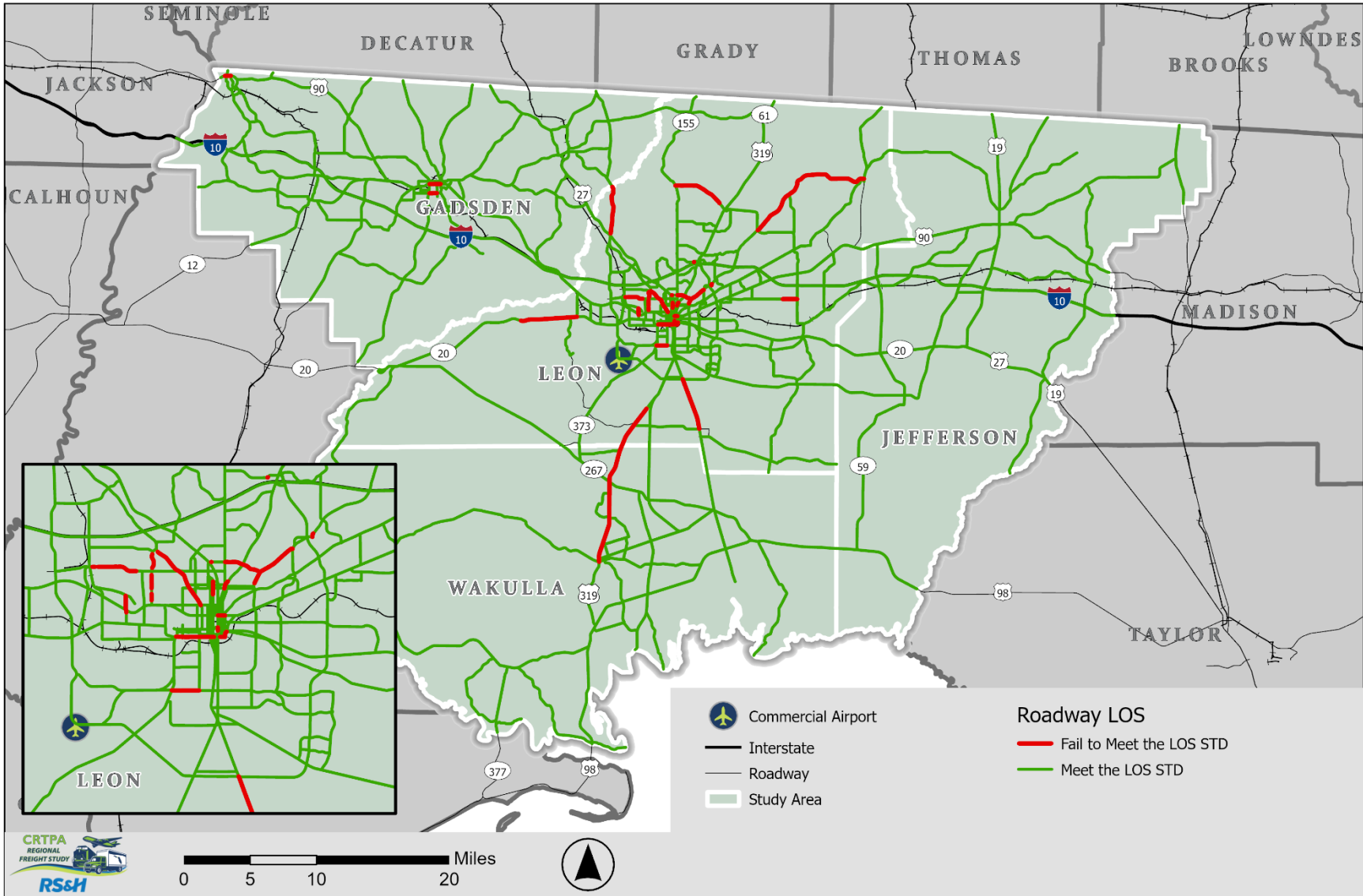
Figure 16: Corridors Failing to Meet LOS
